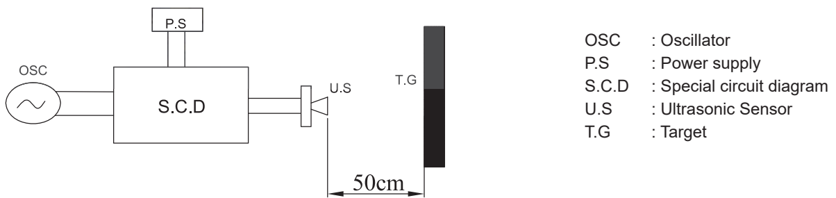
Echo & Rest. Resonant Time test circuit
